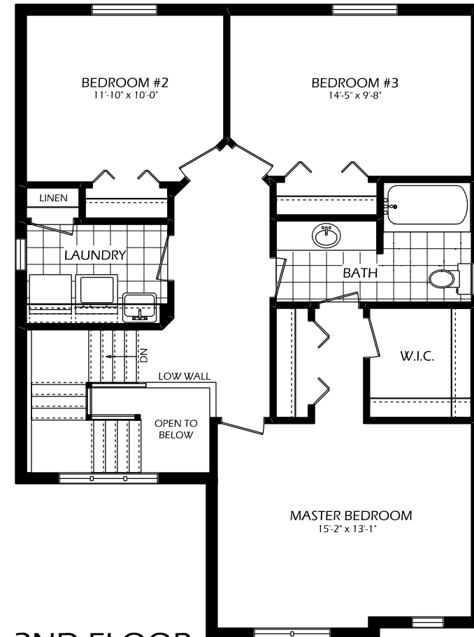
2ND FLOOR 920 SQ. FT. 8' CEILINGS (2ND FLOOR)
