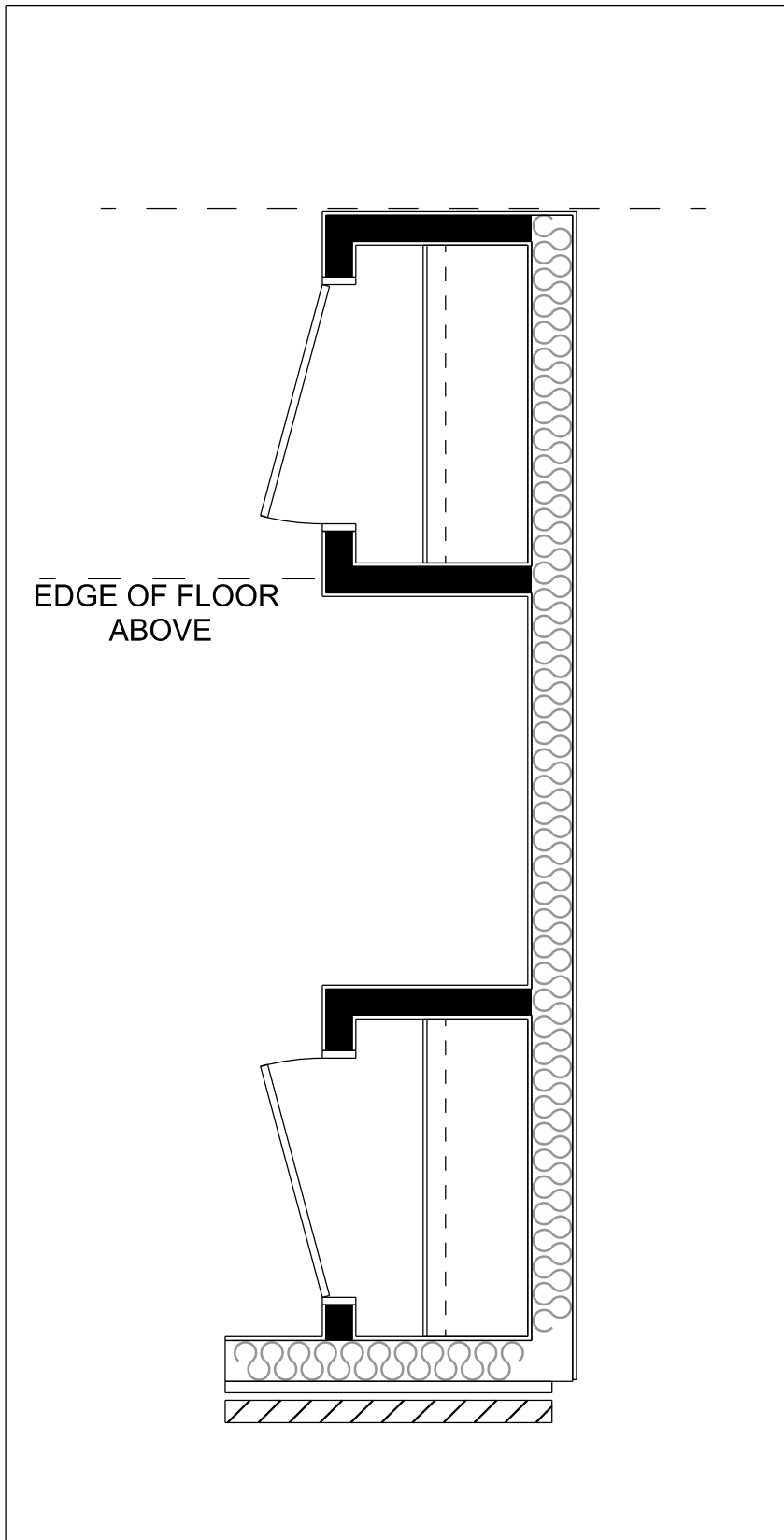
LIVINGSTON OPTIONAL FOYER CLOSET DESIGN(opt#3) 2 SMALLER CLOSETS WITH SWING DOORS AND SPACE BEWTEEN FOR OPTIONAL BENCH
