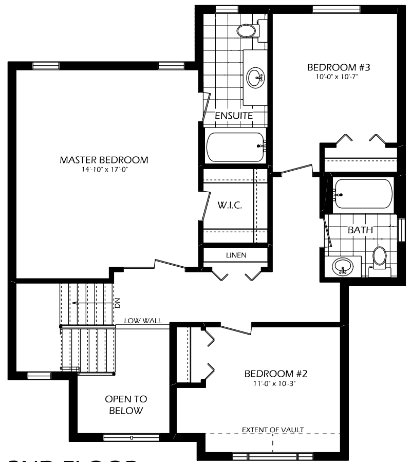
2ND FLOOR 945 SQ.FT. 8' CEILINGS (ON 2ND FLOOR)
