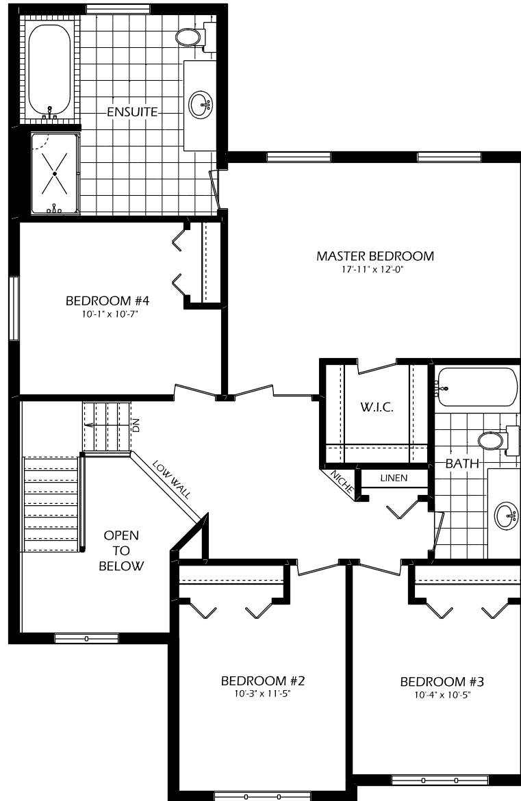
2ND FLOOR 1201 SQ. FT. 8' CEILINGS (2ND FLOOR)
