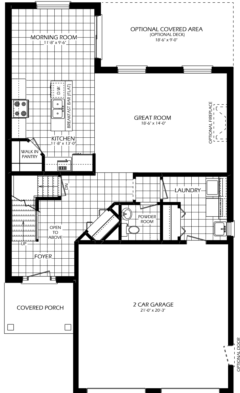
MAIN FLOOR 969 SQ. FT. 8' CEILINGS (ON MAIN FLOOR)
