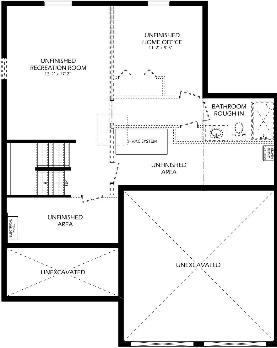
BASEMENT
