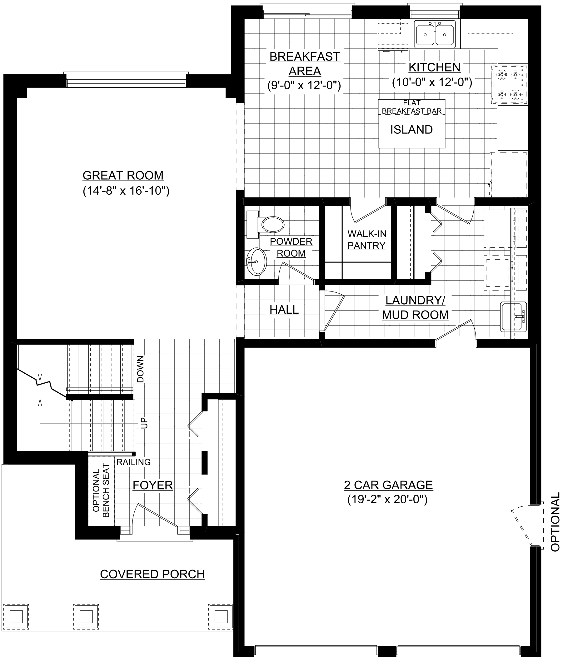
MAINFLOOR PLAN
