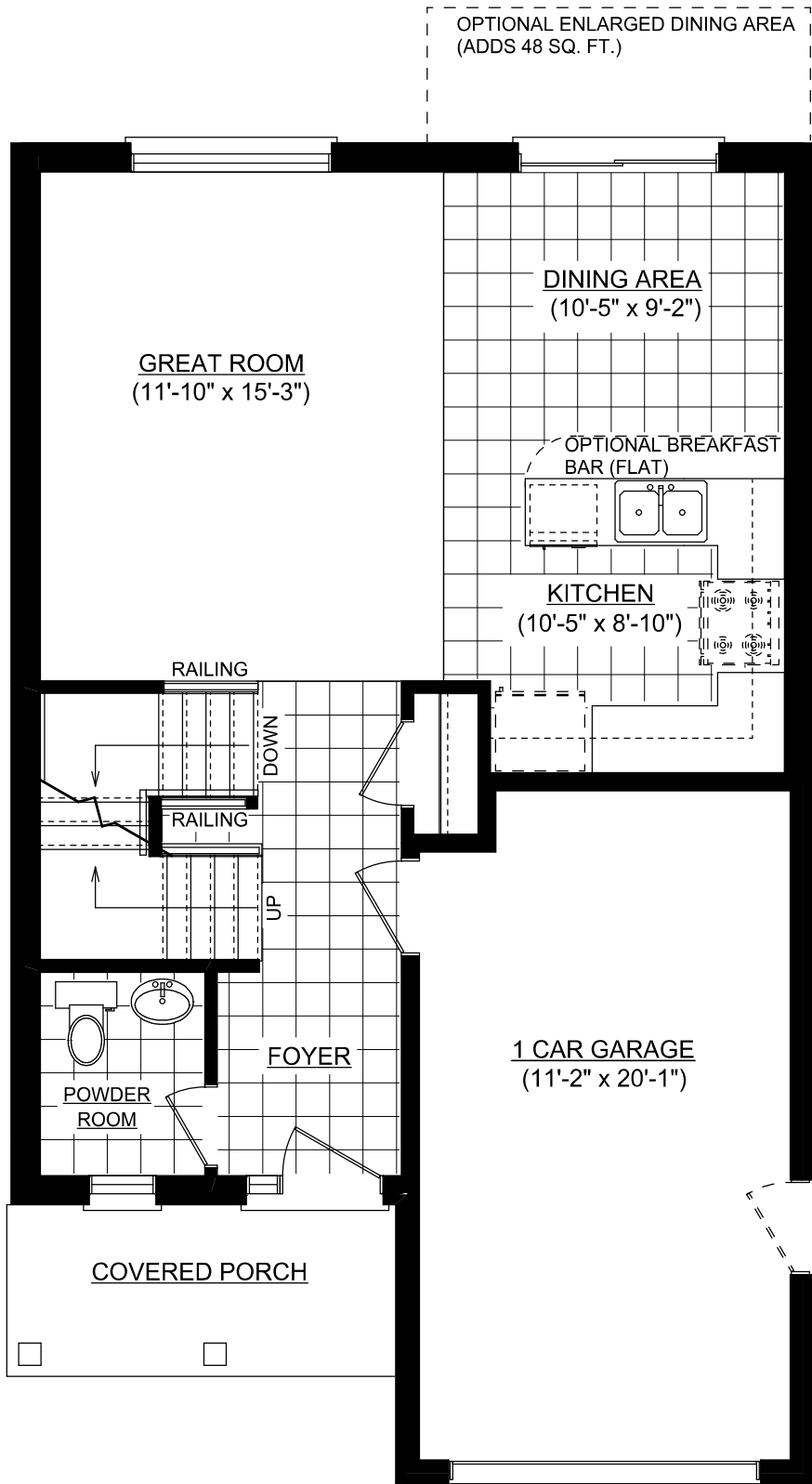
MAINFLOOR PLAN
