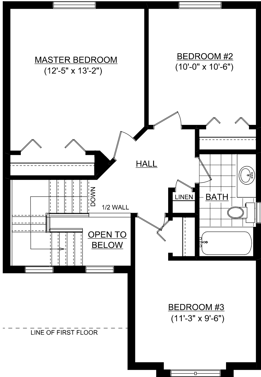
2ND FLOOR PLAN MASTER @ REAR
