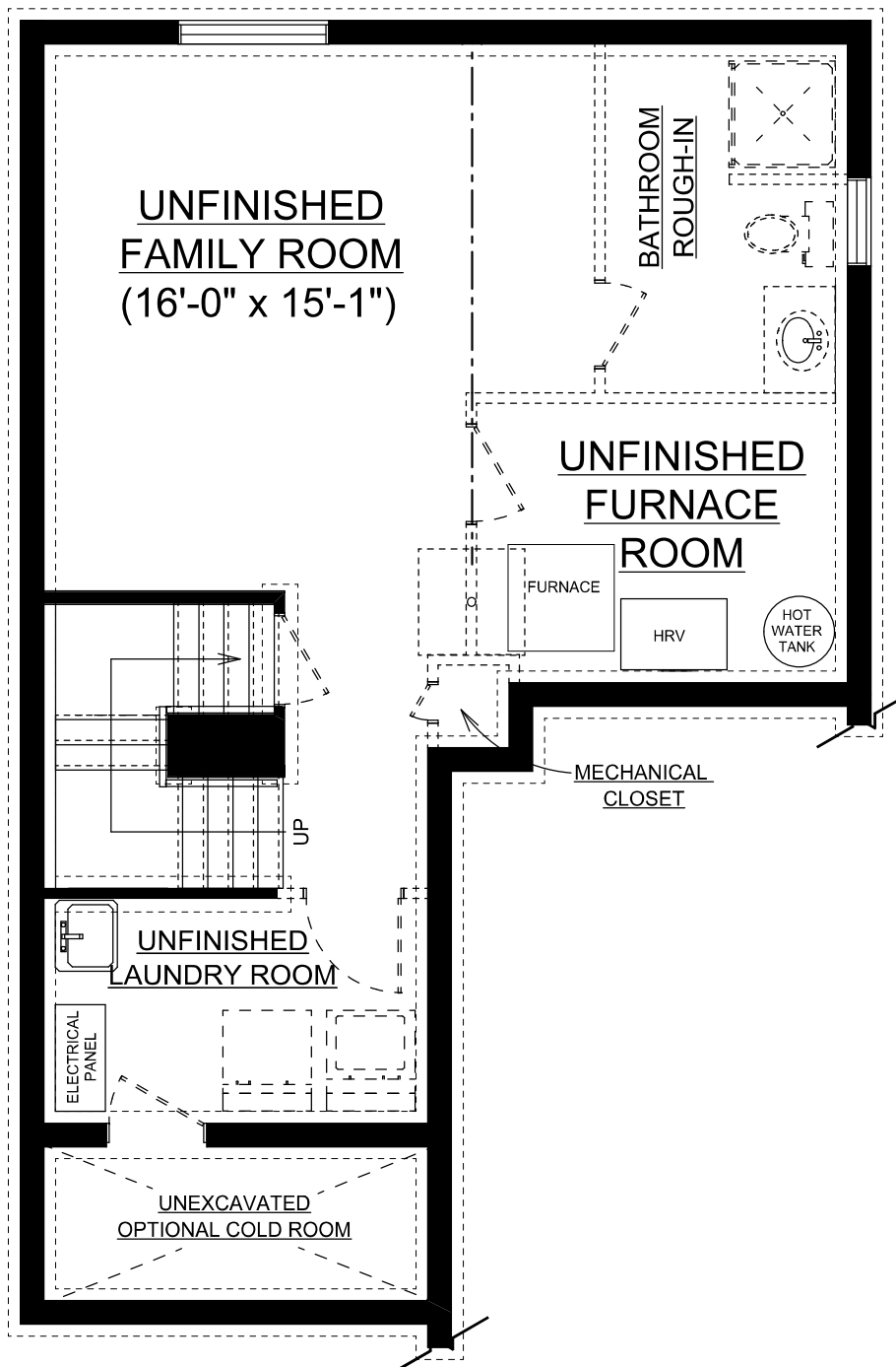
BASEMENT PLAN
