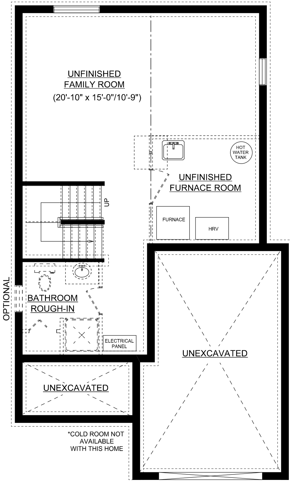
BASEMENT PLAN
