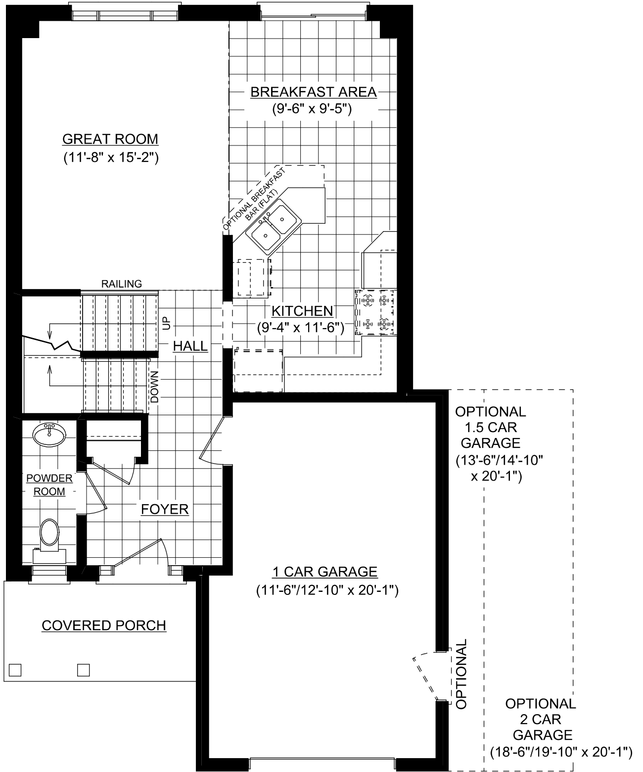
MAINFLOOR PLAN
