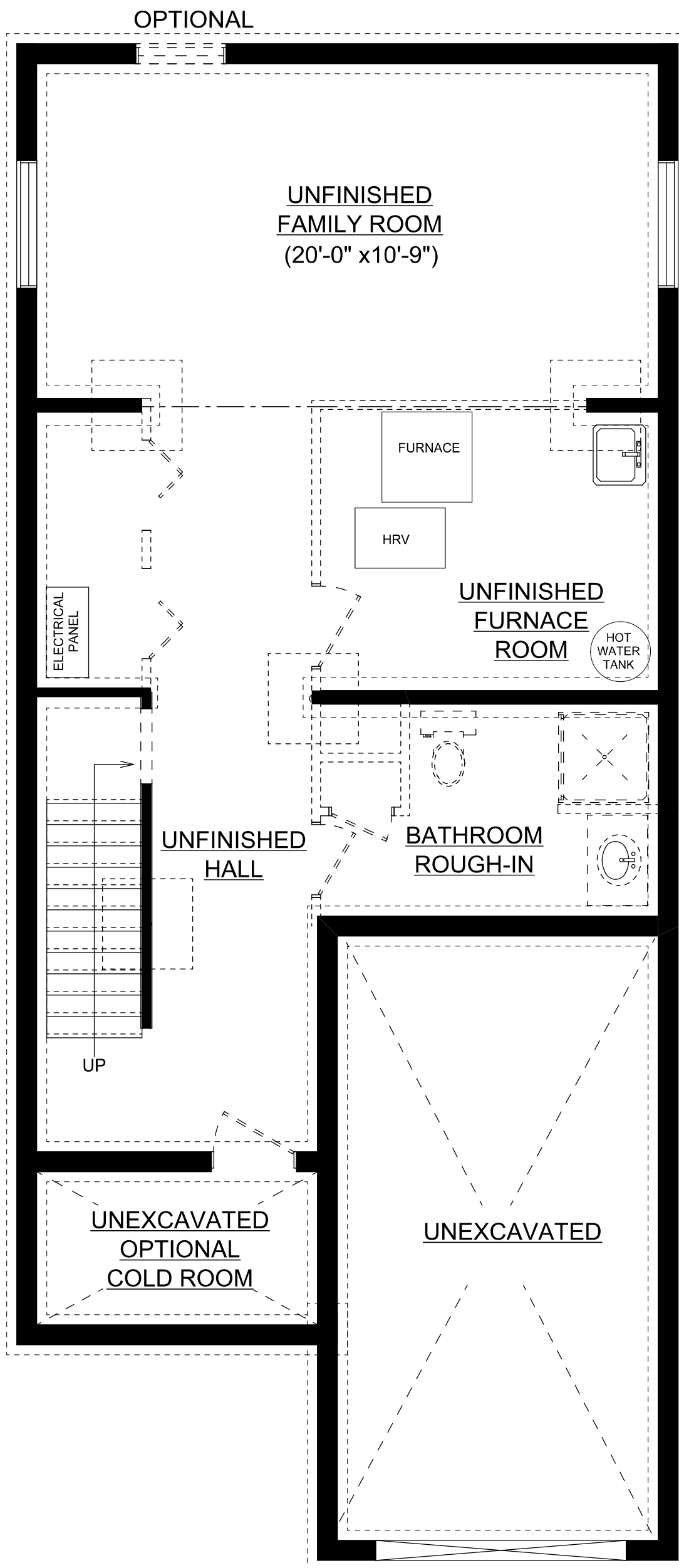
BASEMENT PLAN
