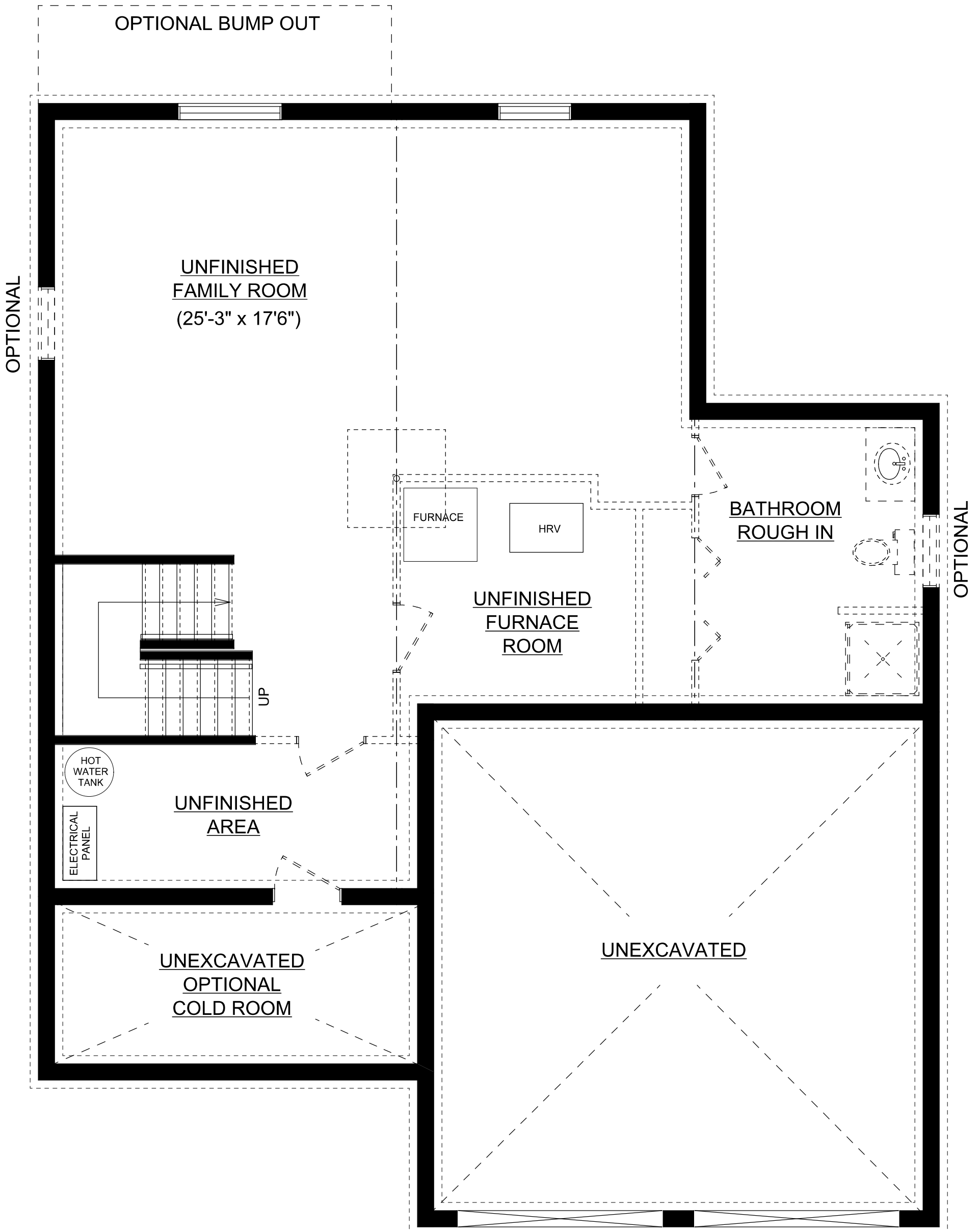
BASEMENT PLAN
