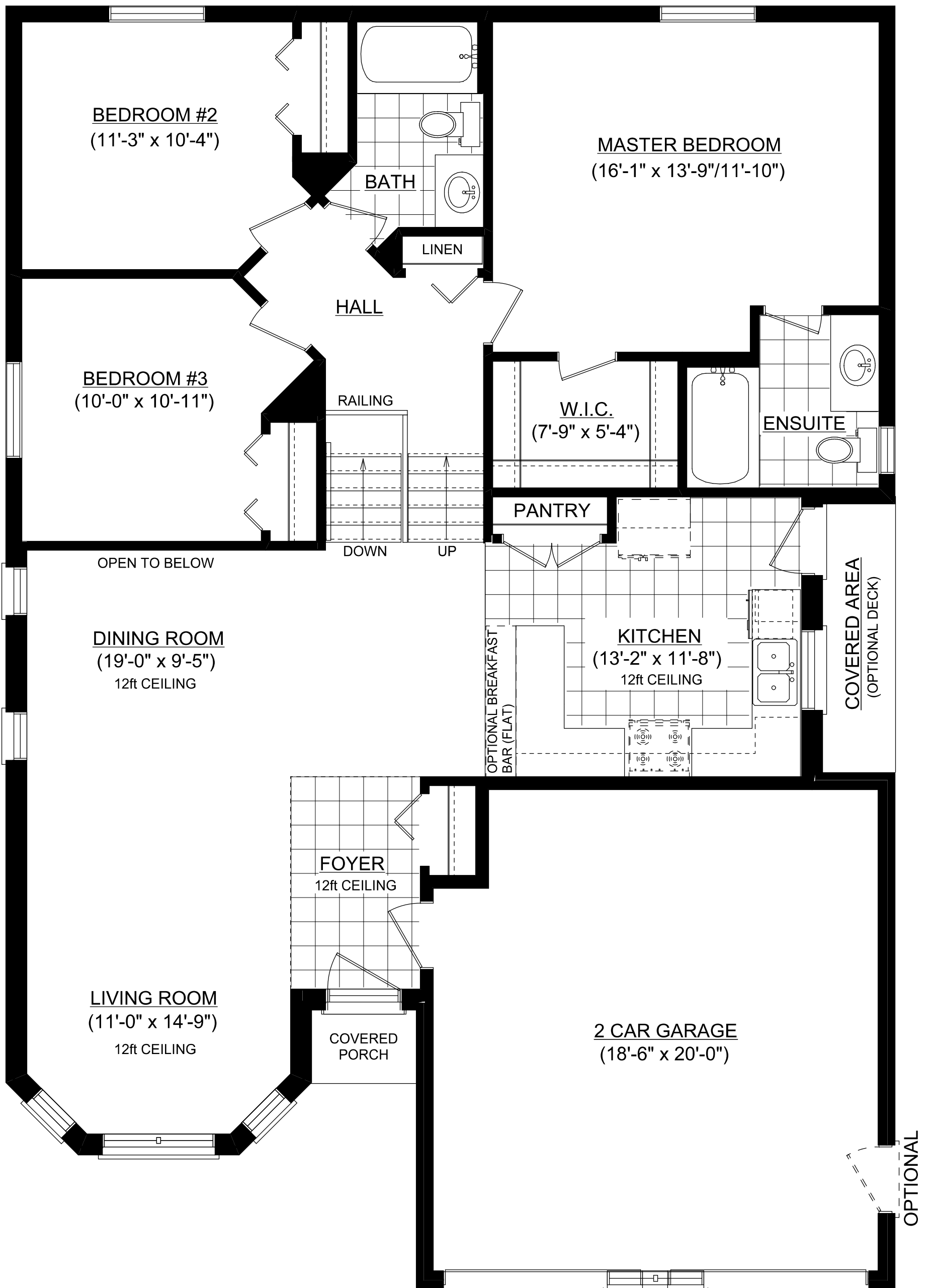
MAINFLOOR PLAN
