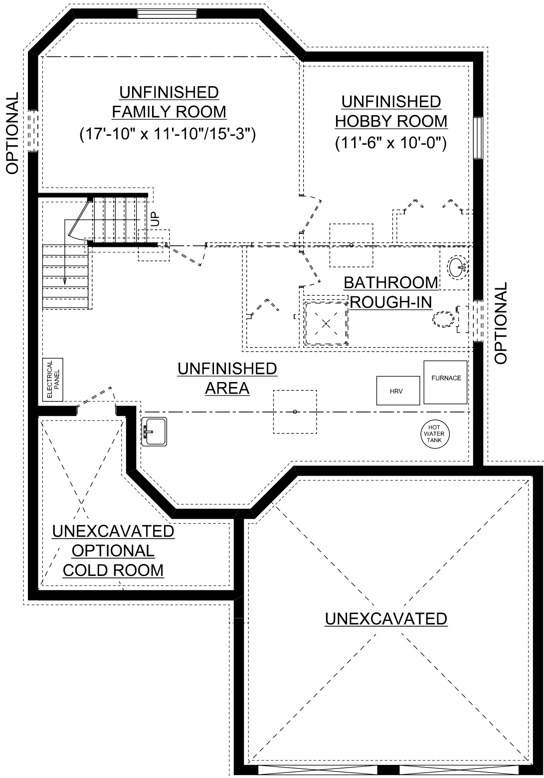
BASEMENT PLAN
