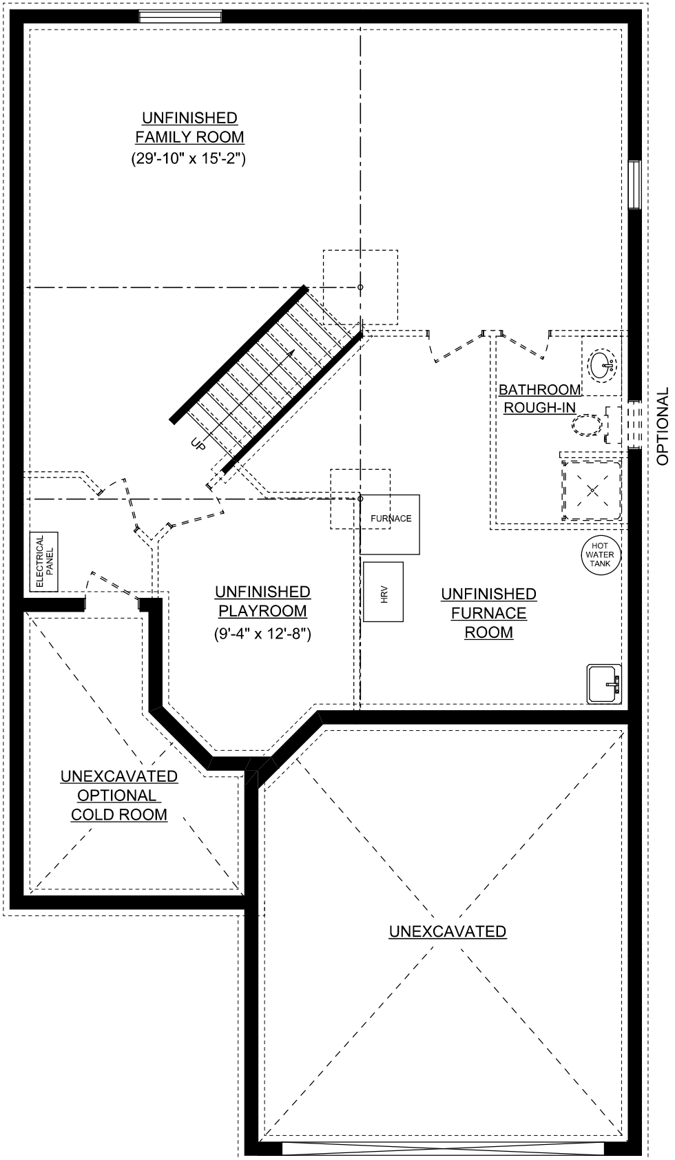
BASEMENT PLAN
