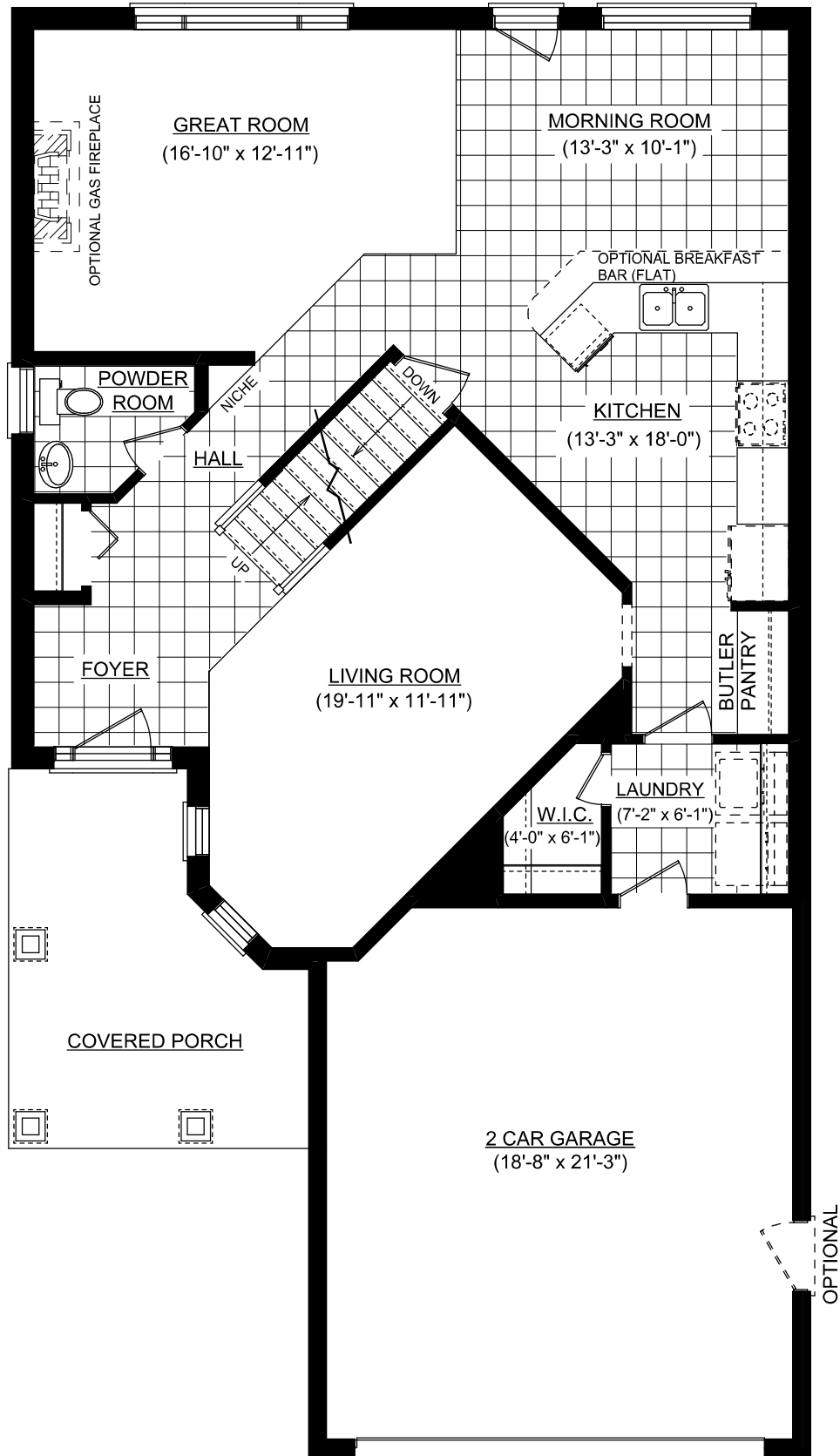
MAINFLOOR PLAN
