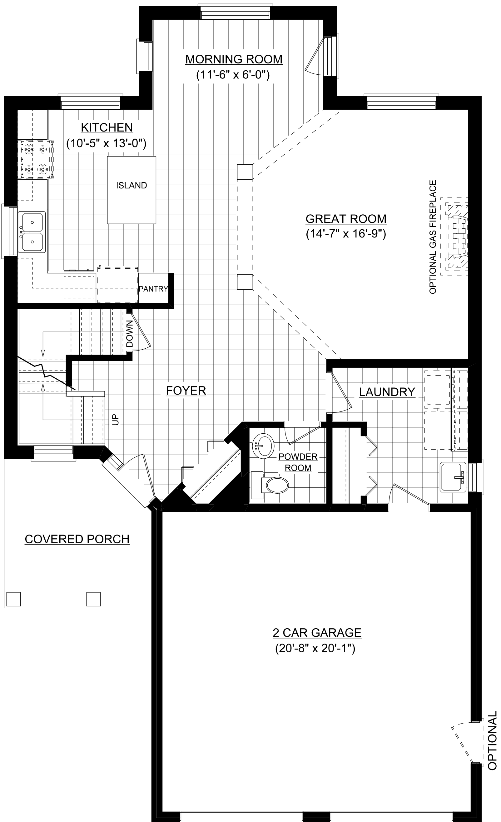
MAINFLOOR PLAN
