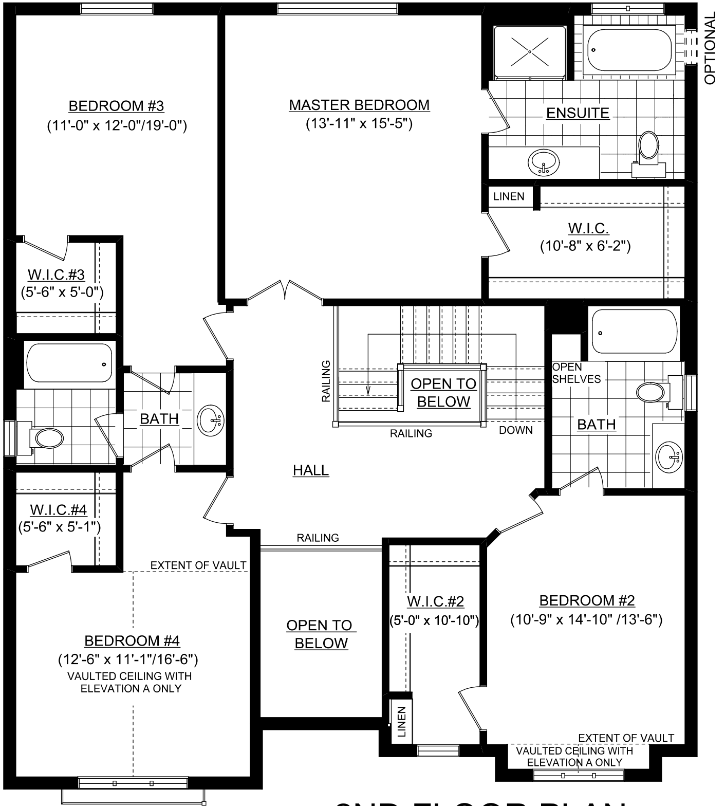
2ND FLOOR PLAN 3 BATHROOM OPTION
